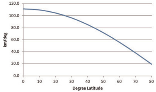
Figure 11. Comparisons of the arc length for one degree of longitude ( dL ) at various latitudes (in kilometres) based on WGS84 ellipsoid parameters.
